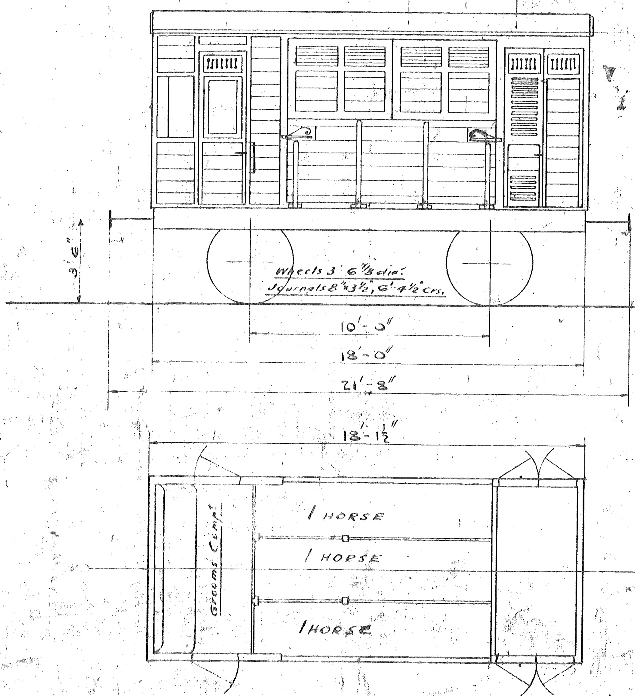
C. L. C. FOUR-WHEELED HORSE BOX.
